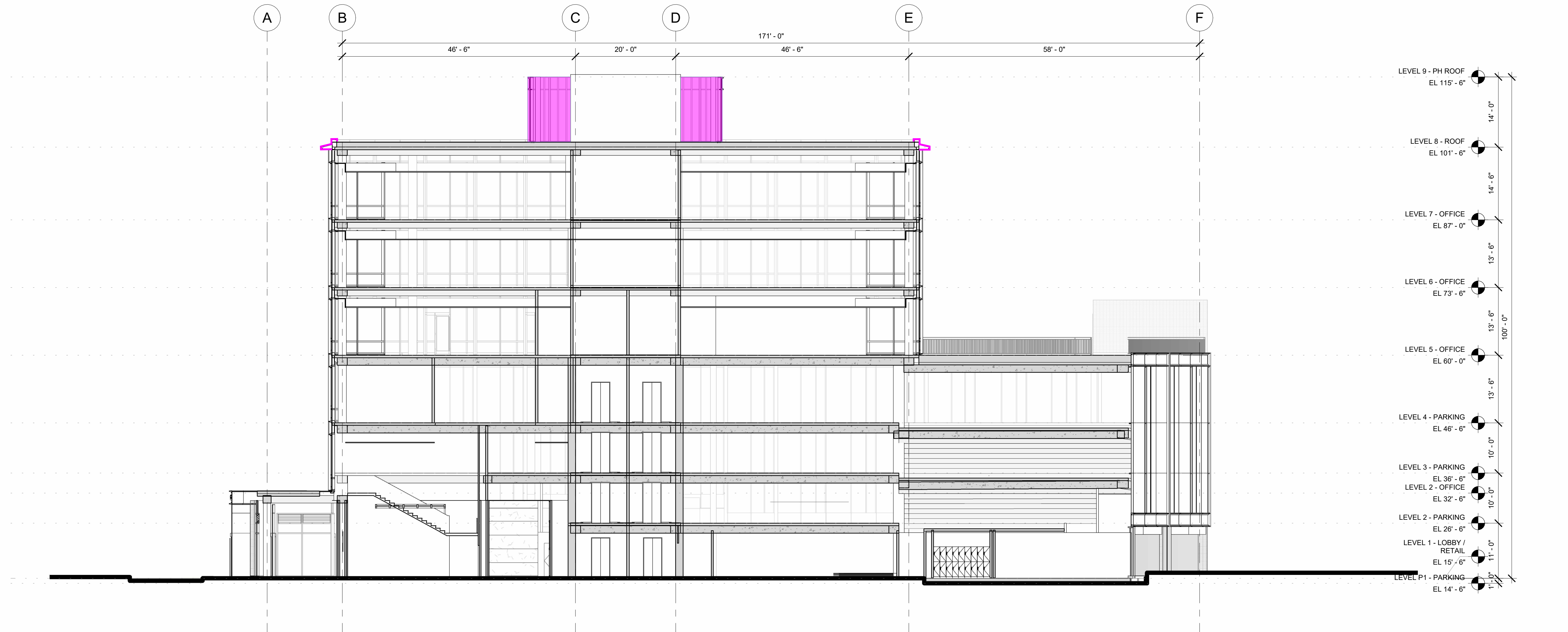
2 N-S BUILDING SECTION - B 3/32" = 1'-0"
